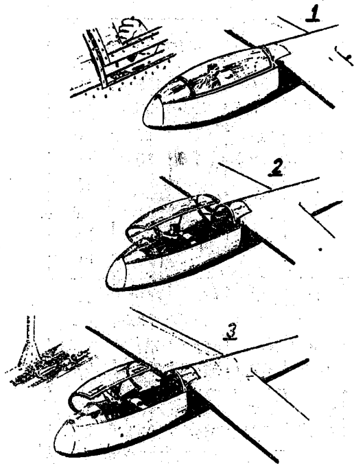
Fig. 11. Jettisoning of cockpit hood of sailplane not fitted with hood emergency release mechanism.
