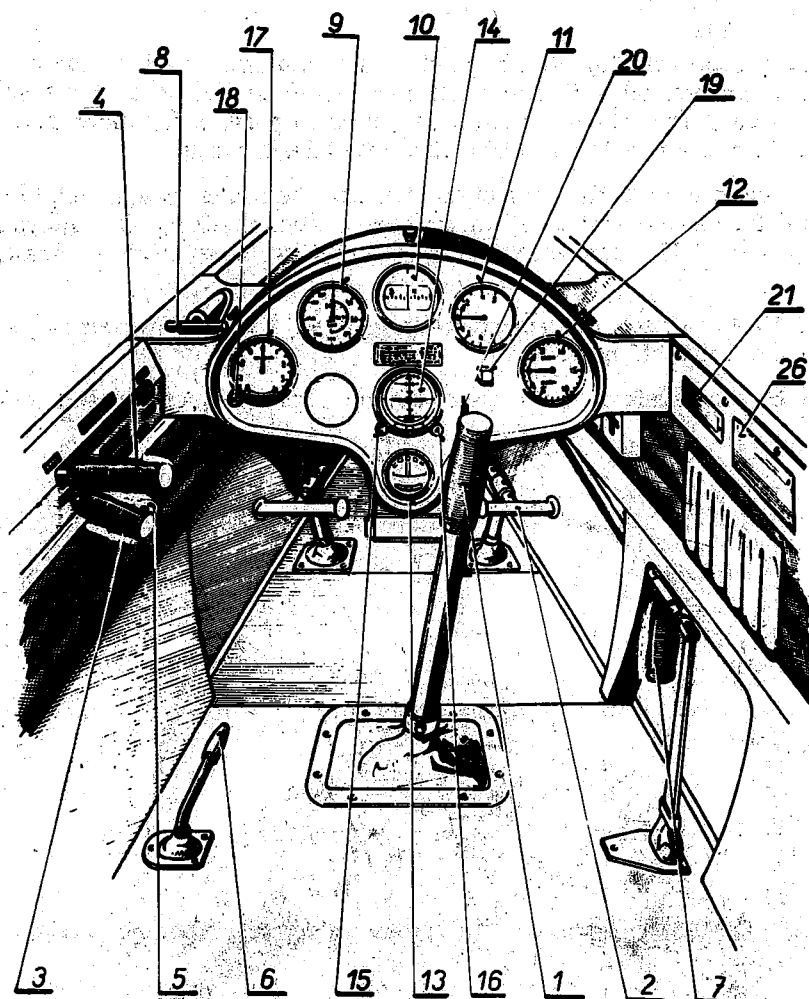
Fig. 2. Rear Cockpit (including optional extra instruments)
