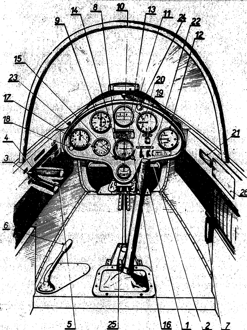
Fig. 1. Front Cockpit (including optional extra instruments)
